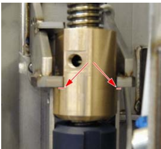
Fig. 22: Inserting the spindle nut mount
