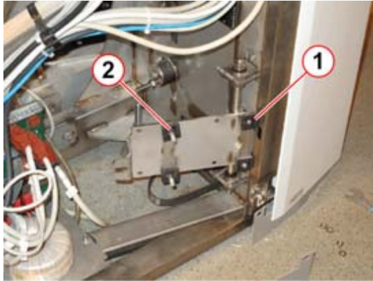
Fig. 29: Mounting plate
